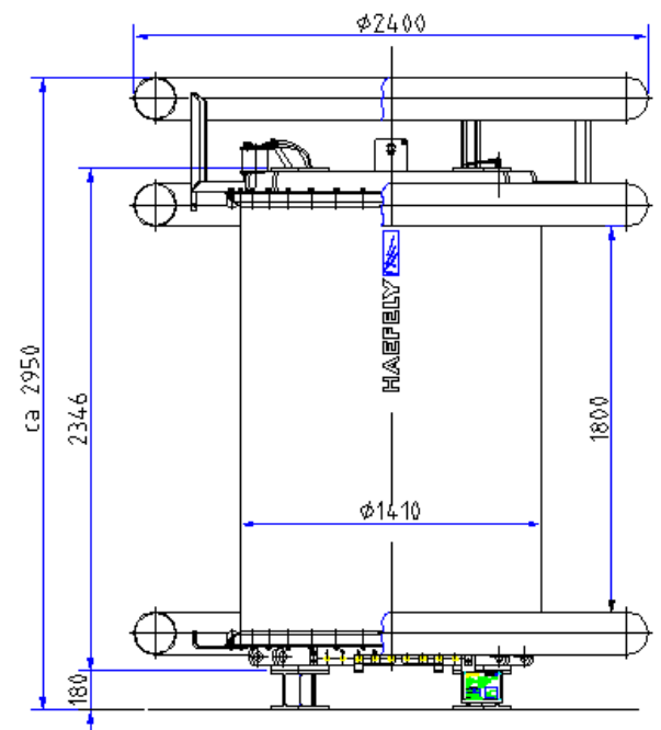
Layout of test transformer 300 kV, 1 A
